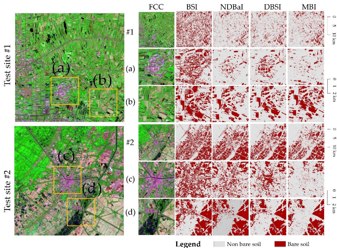
Figure 7. Spatial distribution of bare soil layers extracted from BSI, NDBaI, DBSI, and MBI on entire test sites and zoom-in areas in solid line squares where there were significant differences among the indices compared to FCC images: (a,b) Test site #1, (c,d) Test site #2.
