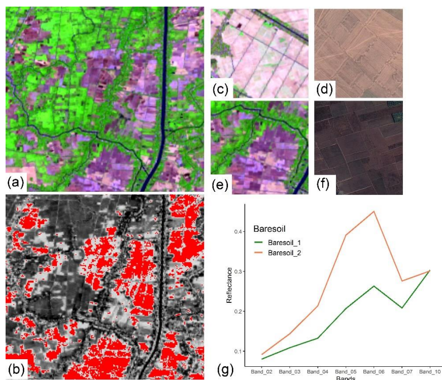
Figure 9. (a) False-color composite (RGB: 6-5-3) at a mixed bare soil area, (b) bare soil classified by the MBI thresholding (red), the remnant bare soil areas are in a bright tone, (c) a fragment of typical dry bare soil (type #2) can be detected by MBI on Landsat 8 image, (d) dry bare soil on Google Earth image, (e) a typical moist bare soil (type #1) is undetectable by MBI on Landsat 8 image, (f) wet bare soil on Google Earth image with darker brown tone compared to dry bare soil, and (g) spectral profiles of dry and wet bare soil.
