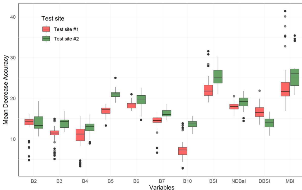
Figure 8. A boxplot shows mean decrease accuracy (MDA) by different Landsat 8 bands and four bare soil indices in random forest classification on the two test sites. Note: Values greater than 50% of MBI are not shown on the plot for better visualization.
