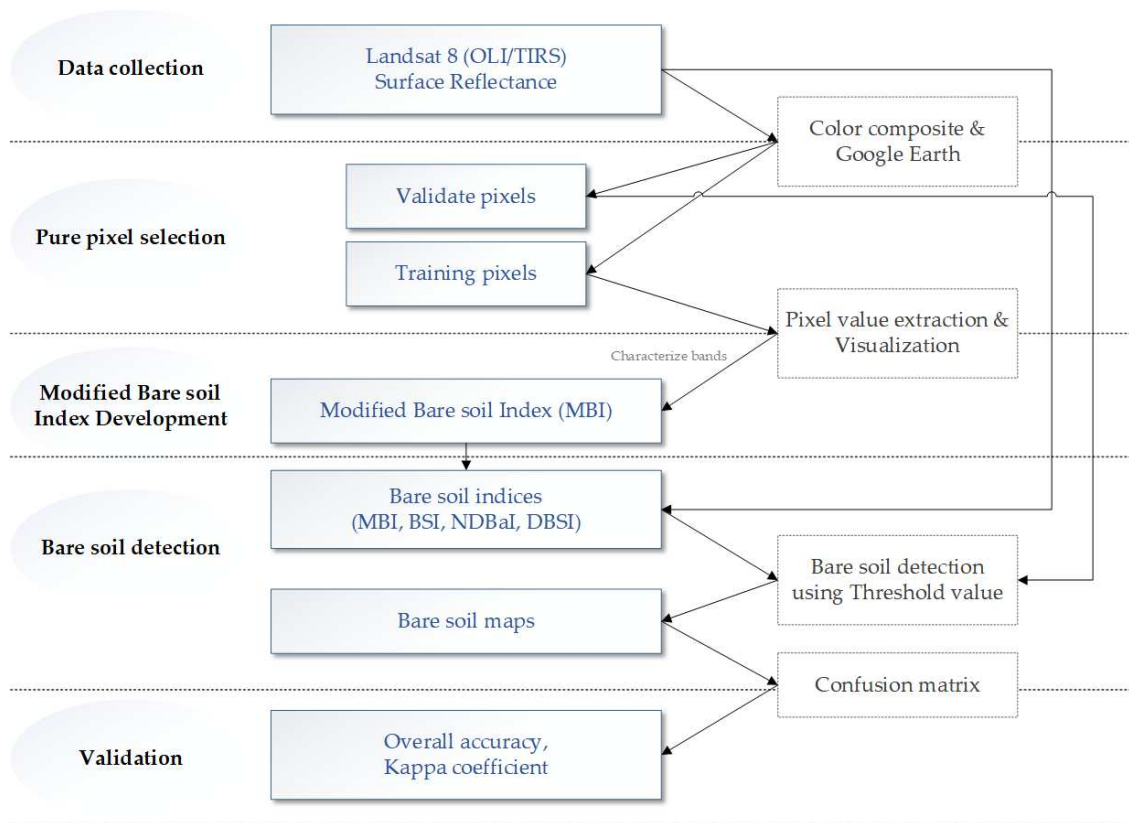
Figure 1. Flowchart showing the detailed research methodology to develop and validate the modified bare soil index.
