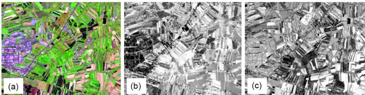
Figure 4. Magnified images (a) false-color composite (RGB: 7-5-3) with pink and purple representing built-up and bare soil, (b) normalized image on SWIR1 and SWIR2 (Equation (1)), which mostly highlights vegetation with bright tone, bare soil in gray and urban areas in black, and (c) three-band bare soil index (Equation (2)) emphasizing bare soil (bright tone), urban features in gray and vegetation in black.
